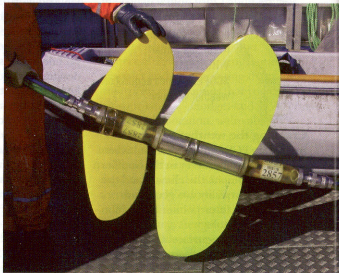
The Q-Fin design deflects streamers by up to six degrees against the natural feather. (Image courtesy of WesternGeco)
